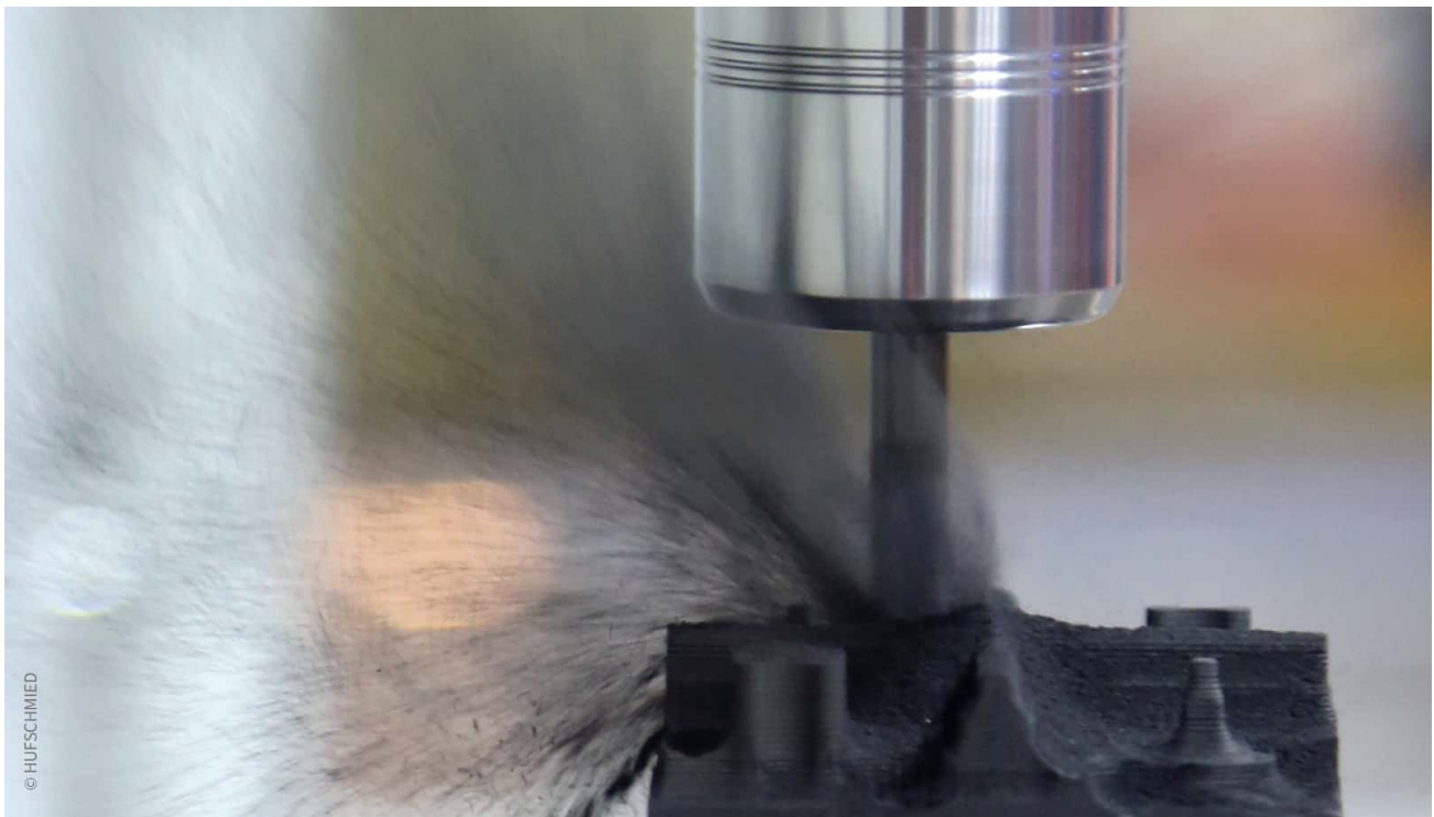
Diamond coatings from CemeCon offer the ideal solution for milling graphite electrodes (Photo: HUFSCHMIED).
